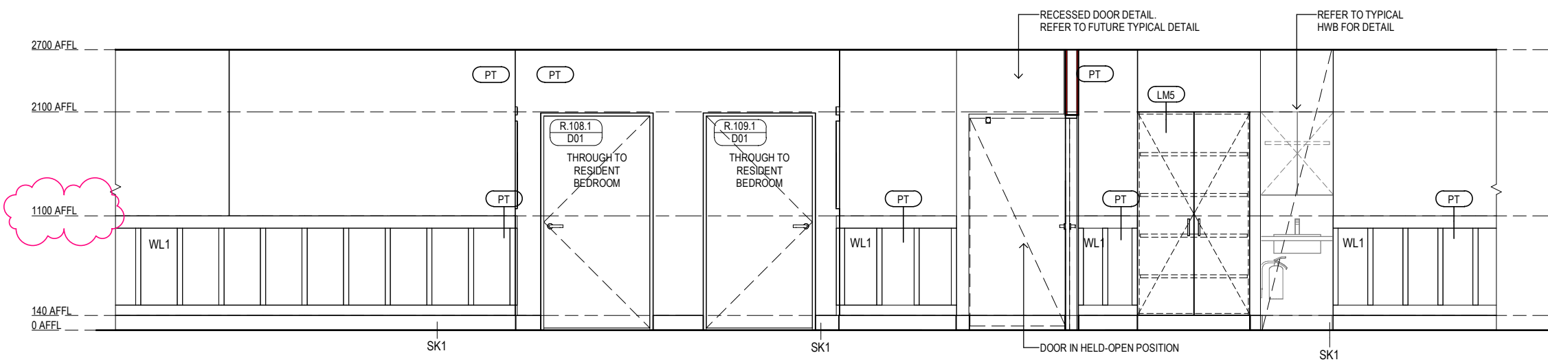
TYPICAL RESIDENT CORRIDOR ELEVATION 5 Scale 1 : 50
