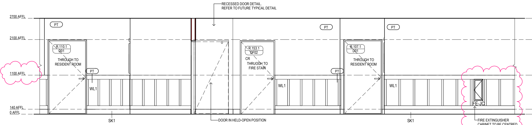
TYPICAL RESIDENT CORRIDOR ELEVATION 4 Scale 1 : 50
